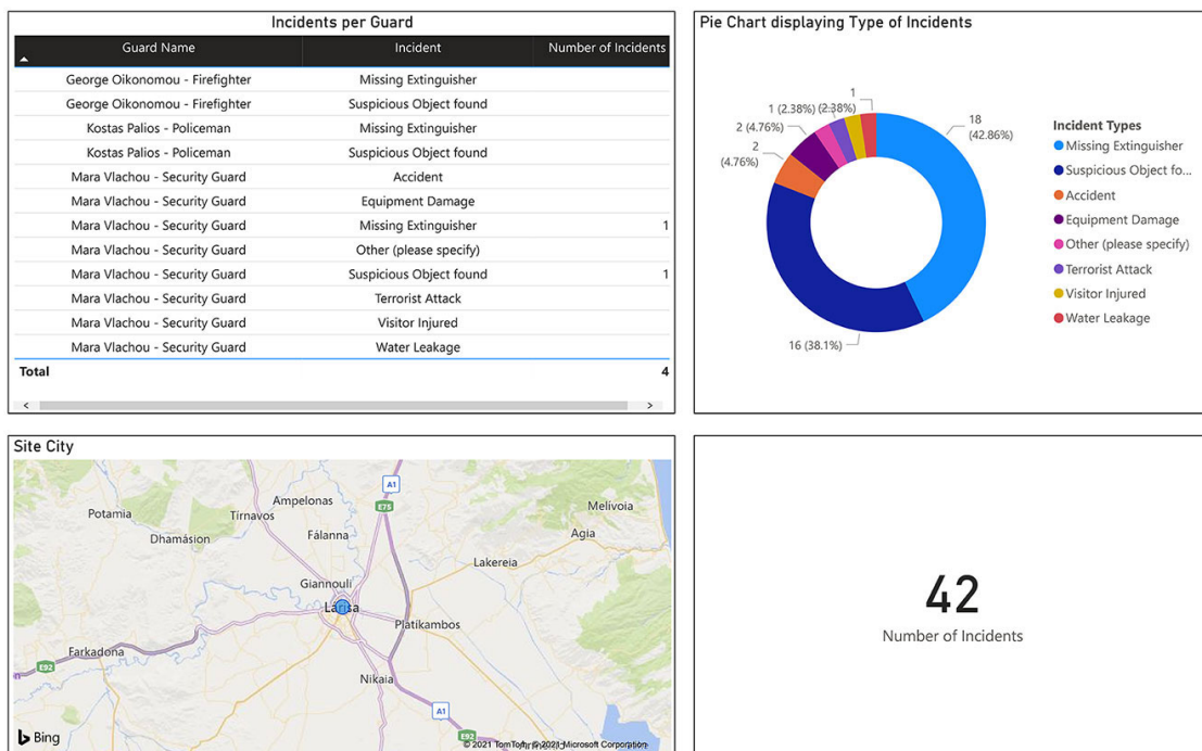
QR-Patrol Dashboard
